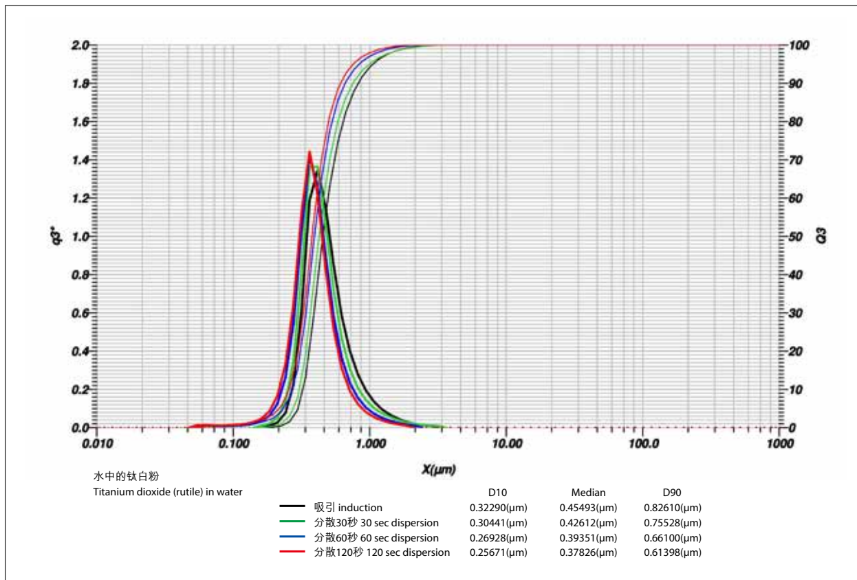
图 3: 钛白粉被吸入后分散 30 秒、60 秒和 120 秒的粒径分布 Figure 3: Particle size distribution titanium dioxide having 30, 60 and 120 seconds of dispersion after induction
